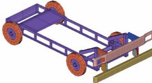
Fig. 3. Modified moving barrier
