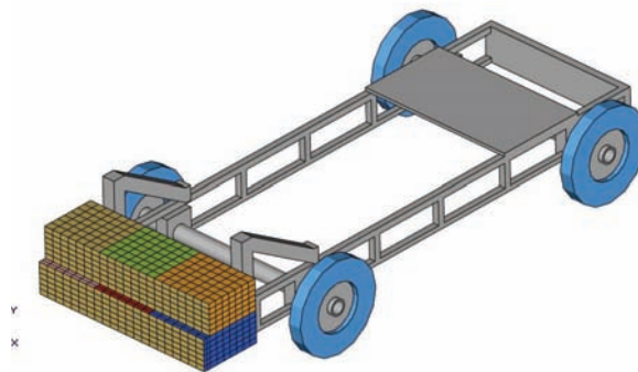
Fig. 2. Original moving barrier
