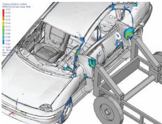
Fig. 7. Moving barrier without lights assembler part – plastic strains
