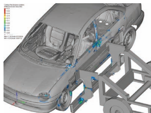
Fig. 8. Plastic Strains – velocity 51km/h, height 300m, position 0, angle 0
