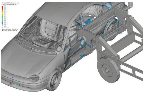
Fig. 7. Moving barrier without lights assembler part – plastic strains
