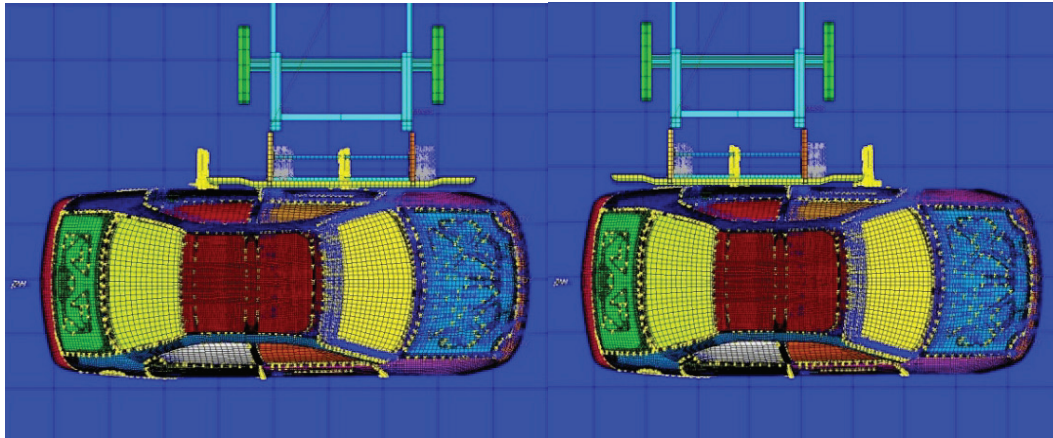
Fig. 5. Position of the moving barrier in the relation to the car
