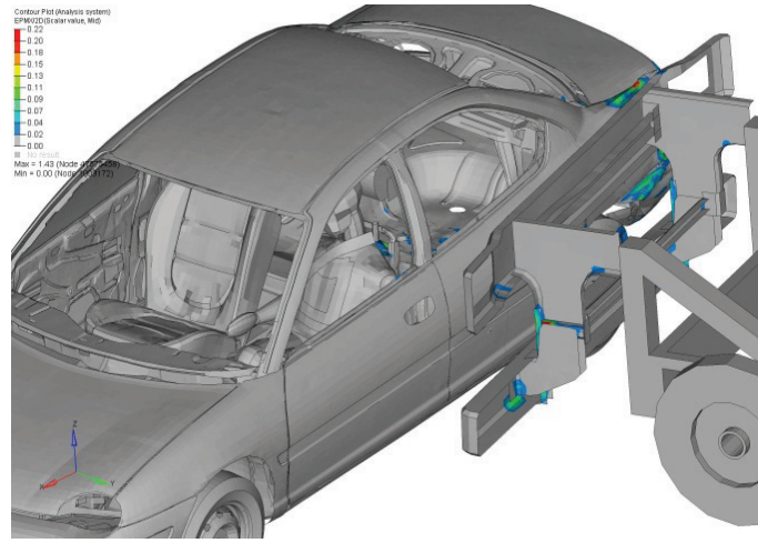
Fig. 11. Plastic Strains – velocity 51km/h, height 300m, position +800, angle -20, Fig. 12. Plastic Strains – velocity 51km/h, height 300m, position -800, angle +20
