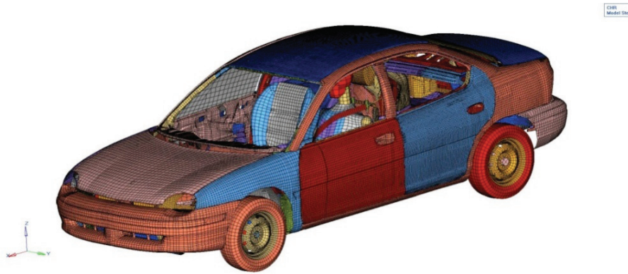
Fig. 1. The Chrysler Neon model with additional driver metal structure seat
